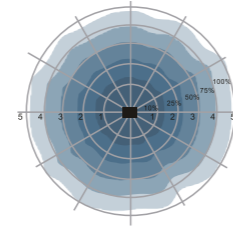
Ceiling mounting pattern(Unit:m) Suggested installation height:2.5-6mm
