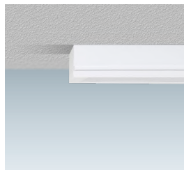
Mounting Bracket: Specially designed extruded seamless aluminium bracket installed behind the luminaire results in easy installation with hanging capability by using proper bracket
